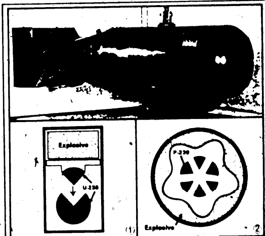
ABOVE are rough diagrams of two types of fission bombs. The first is a uranium-235 gun assembly, which is the type bomb dropped at Hiroshima (pictured above). It contained less than 100 lbs. of uranium but released the equivalent destructive force of 20,000 tons of T.N.T. In this design, one section of U-235 is shot into the other by the use of high explosives to achieve atomic fission. The second type demonstrates the implosion technique and was used in the first "Fat Man" test blast and later at Nagasaki. It requires a high explosive shell to be detonated around two or more pieces of fissionable material, in this case plutonium-239. Sophisticated atomic bombs using the implosion design can be small enough to be carried in a suitcase.
